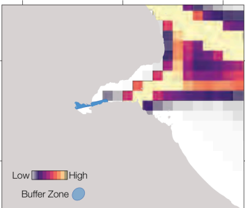
BUNKER or TANKER density (mean count)
