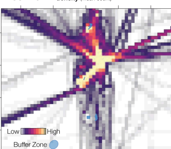
PASSENGER density (mean count)
