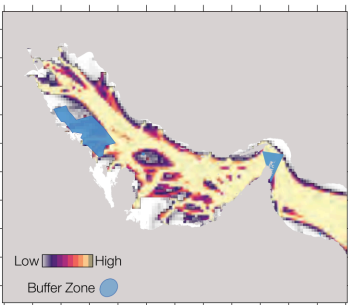
CARGO density (mean count)
