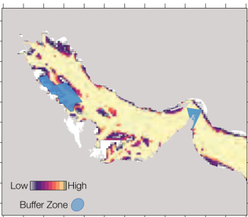
CARGO or TANKER density (mean count)
