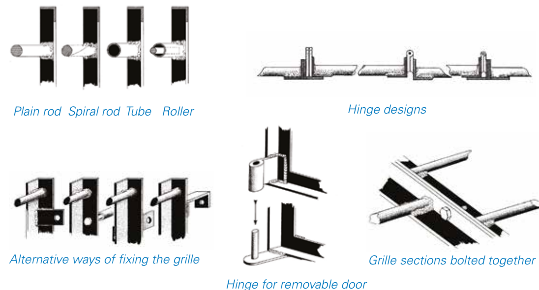
Figure 4. Grille fabrication details.
