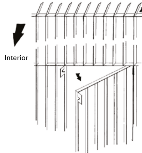
Detail: orientation of the door and the ends of the bars.
