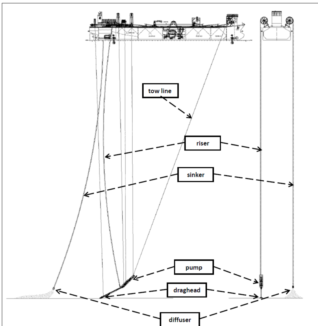
Figure 4. Diagram of the CRP mining proposal. (Source: Figure 5, Evidence from Gerard Van Raalte for CRP, 28 August 2014)
