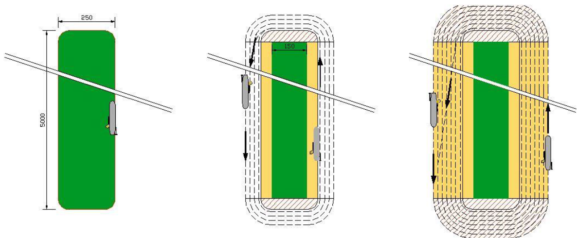
Figure 5. Mining pattern – “spiralling out”. The green area is not mined and the yellow areas are mined or have sediment deposited directly on them. (Source: Statement of Evidence from Gerard Van Raalte for CRP, Figure 8)
