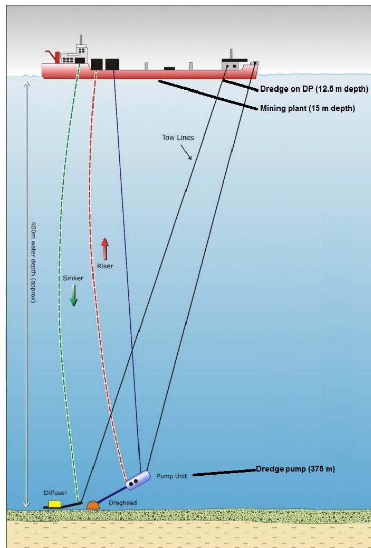
Figure 13. Image of dredge concept with location (depth) of sources used in modelled scenarios. (Source: Figure 3 of JASCO report attached to Statement of Evidence of Dr Darlene Ketten for CRP, 7 October 2014)
