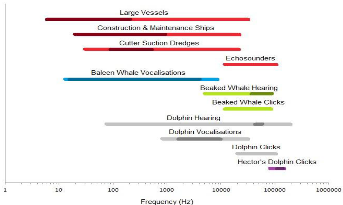
Figure 12. Comparison of marine megafauna hearing ranges with anthropogenic sources. Darker sections of marine mammal hearing ranges indicate peak hearing ranges, range of vocalisations (Johnson 1967, Kastelein et al. 2003, Mellinger et al. 2007, Popov et al. 2007, Houser et al. 2008, Nachtigall et al. 2008, Dawson 1990). Darker sections of anthropogenic sources of noise (red bars) indicate main energy ranges, echo sounders are variable (Götz et al. 2009, Thomsen et al. 2009, CEDA 2011, Robinson et al. 2011). (Source: Figure 1, Statement of Evidence of Simon John Childerhouse for the Crown, 17 September 2014)
